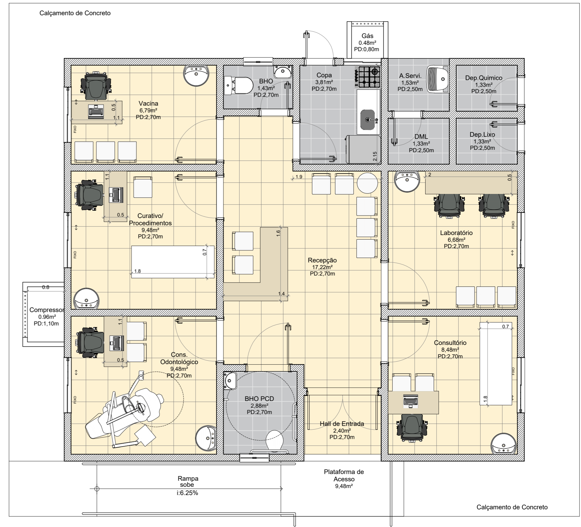
LAYOUT UBS CANOPUS ESCALA - 1:50
